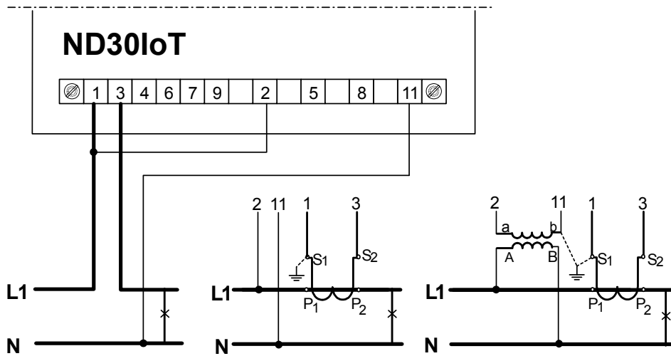
Fig. 4. Meter connections
