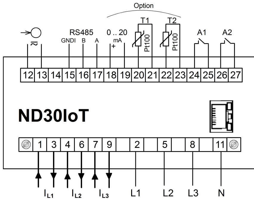
Fig. 4. Meter connections
